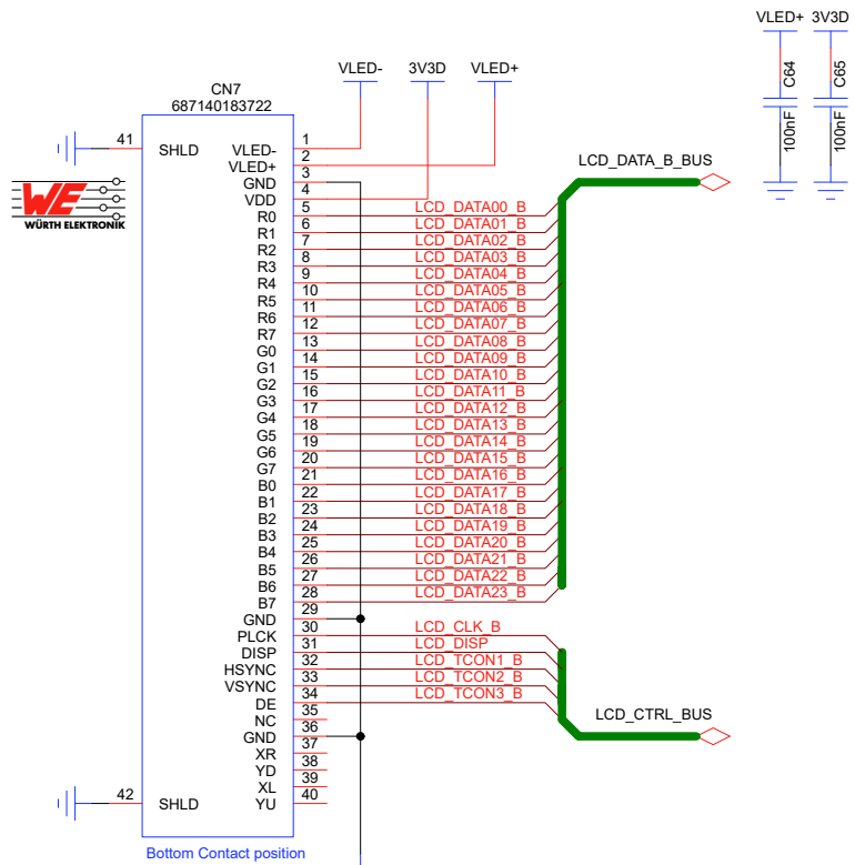
LCD CONNECTOR
